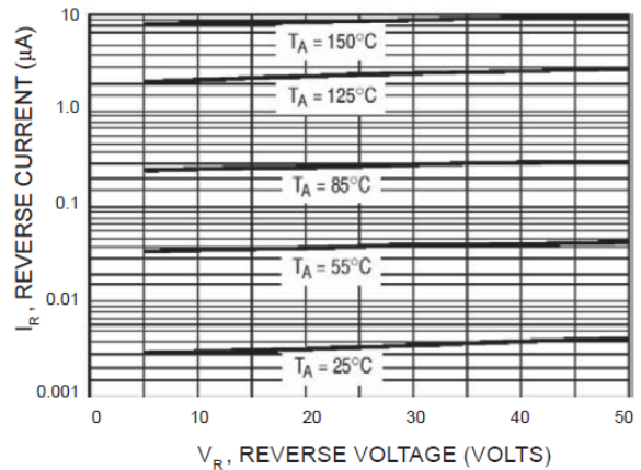
Figure 3. Leakage Current
