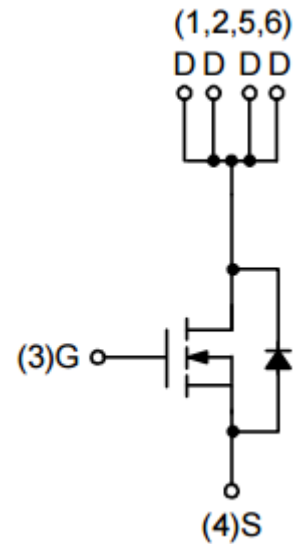
N-Channel MOSFET
